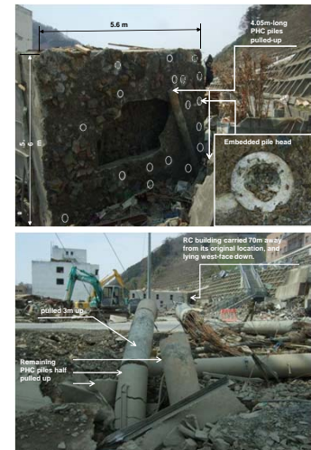
Fig.3 Onagawa town was one of the most seriously tsunami-engulfed towns/cities along the Sanriku coast line. It was shocking that buildings with pre-stressed high-strength concrete piles were uprooted at several locations in Onagawa, all the more pile-supported RC and/or steel-frame structures had been considered to be possibly good for tsunami shelters.
