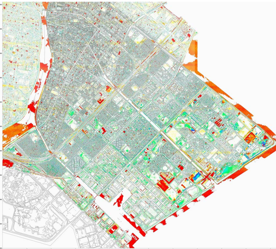
Fig.2 Soil subsidence map of Urayasu:
