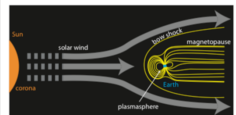
Fig.3 Solar wind and Earth's magnetic field
