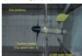
Collision Risk of Marine Animal to Turbine Blades Observing collision and behavior of fish considering similarity law
