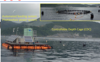
Controllable Depth Cage and Automated Feeding System (Onagawa Bay) Controllable depth cage (CDC) can be installed at any depth.
