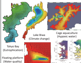
Numerical Simulation Using Hydrodynamic and Ecosystem Coupled Model
