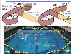
Automated Fish-guiding System Human-saving and labor-saving of net-hauling operation
