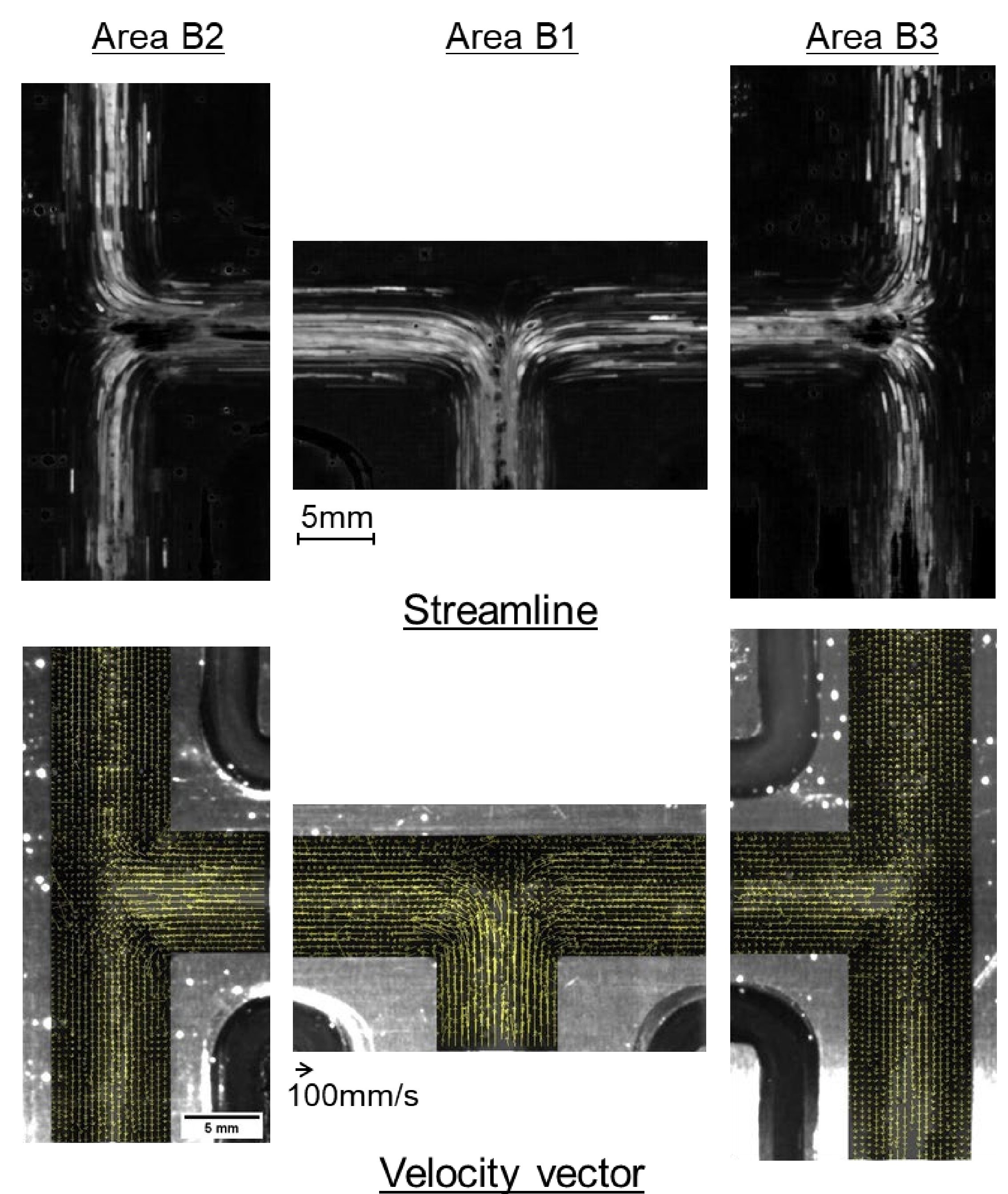
Visualization Analysis of Flow Phenomena at Split Portion in Hot-Runner Manifold
