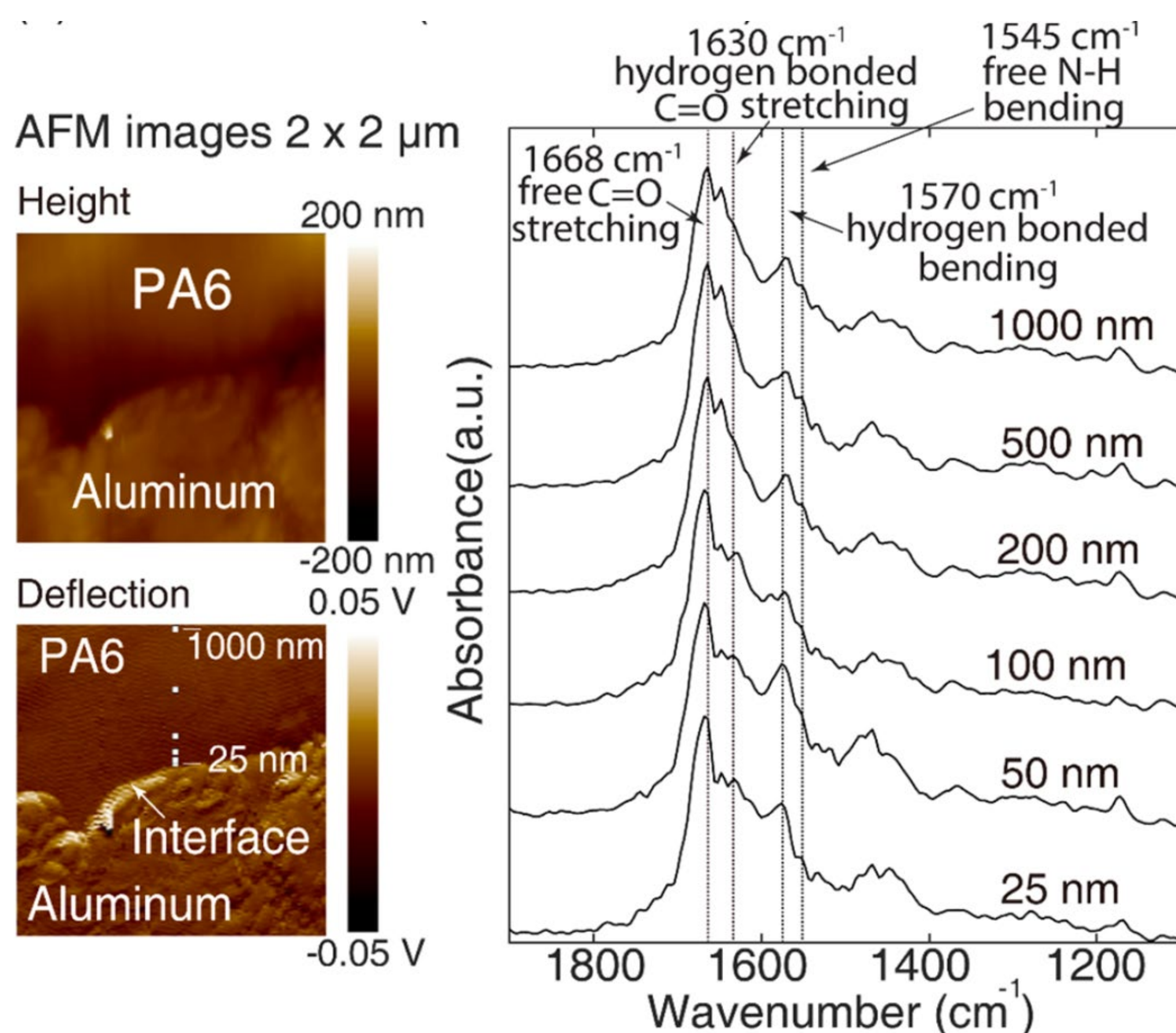
Hydrogen Bonding Spectra at the Interface of Al/PA6 Molding Joint
