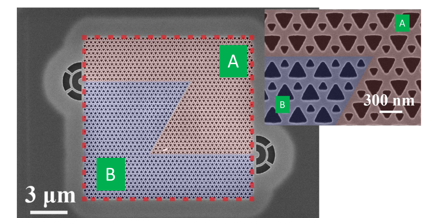
Topological optical waveguide using valley photonic crystal structure
