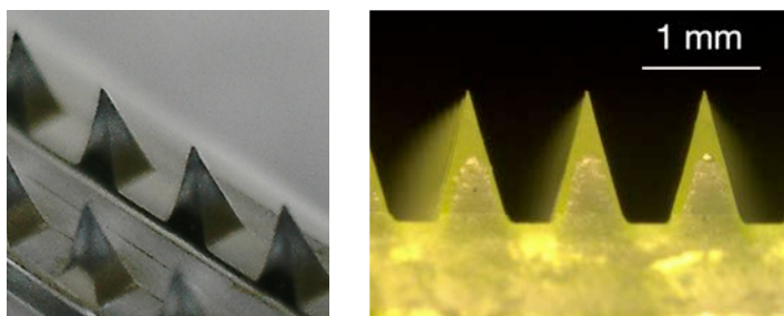
Bio-dissoluble Microneedle Patch for DDS and Sensing
