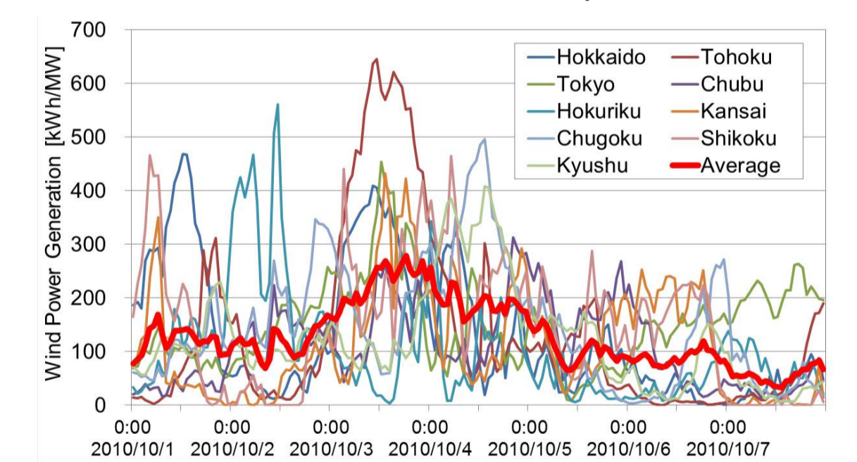
Variation of Wind Power Generation
