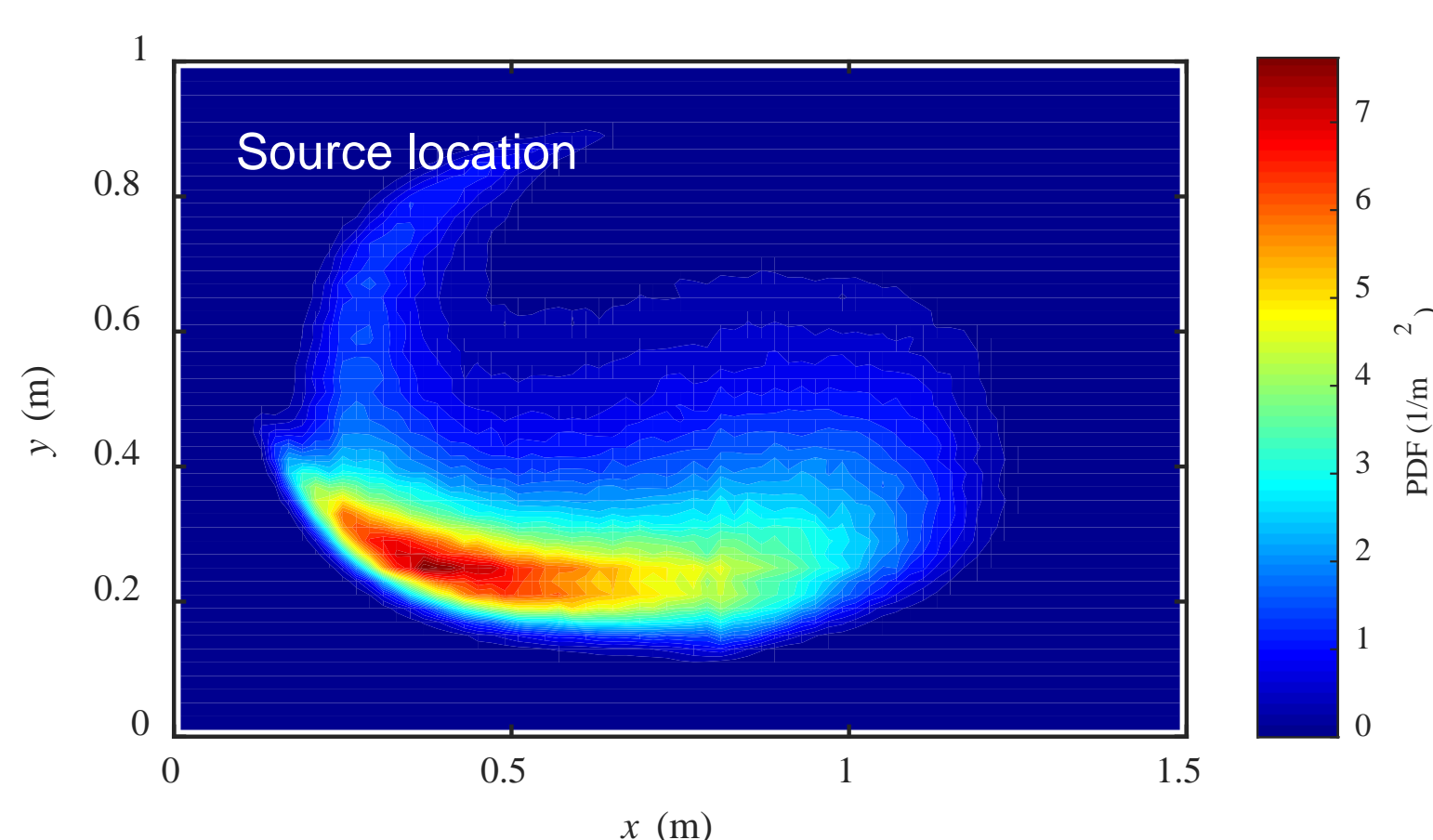
Inverse analysis of unknown pollutant source
