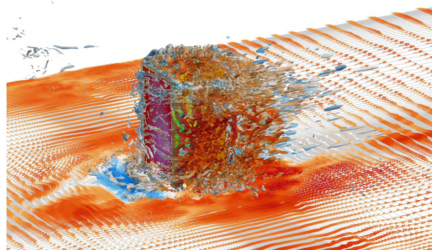
Computational simulation of airflow around building
