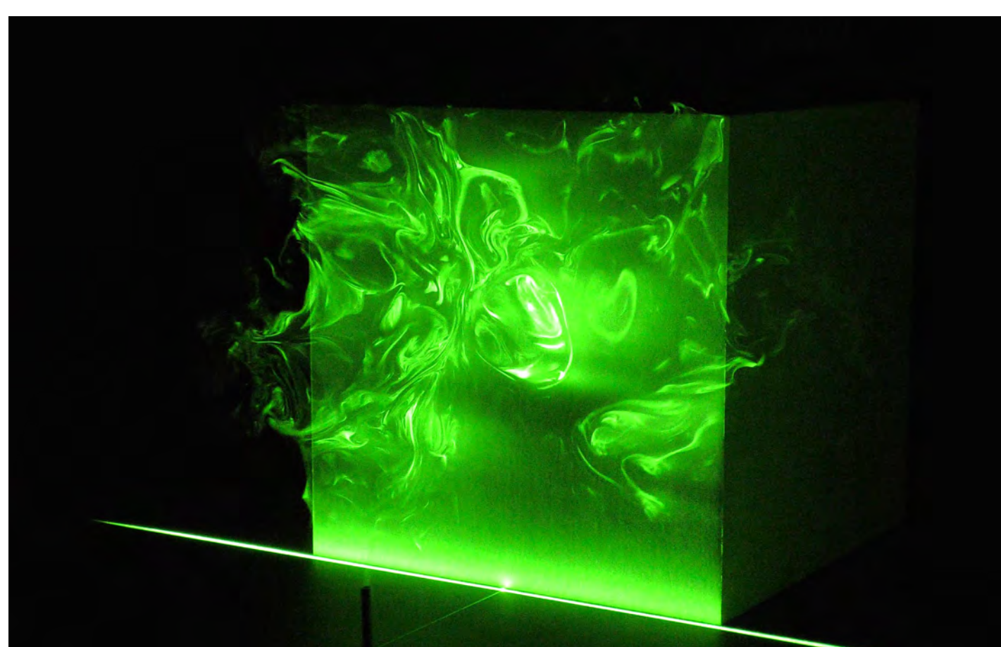
Visualization of pollutant dispersion in wind tunnel
