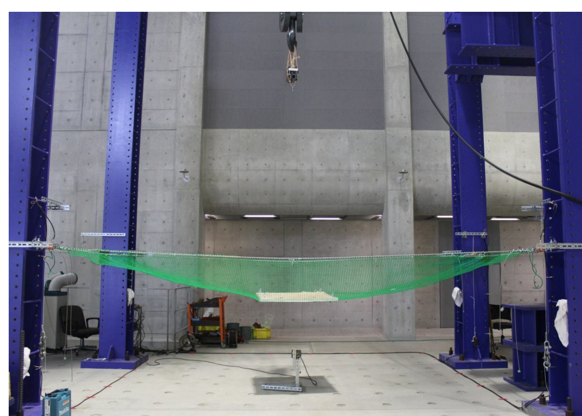
Real-scale tests of the safety net
