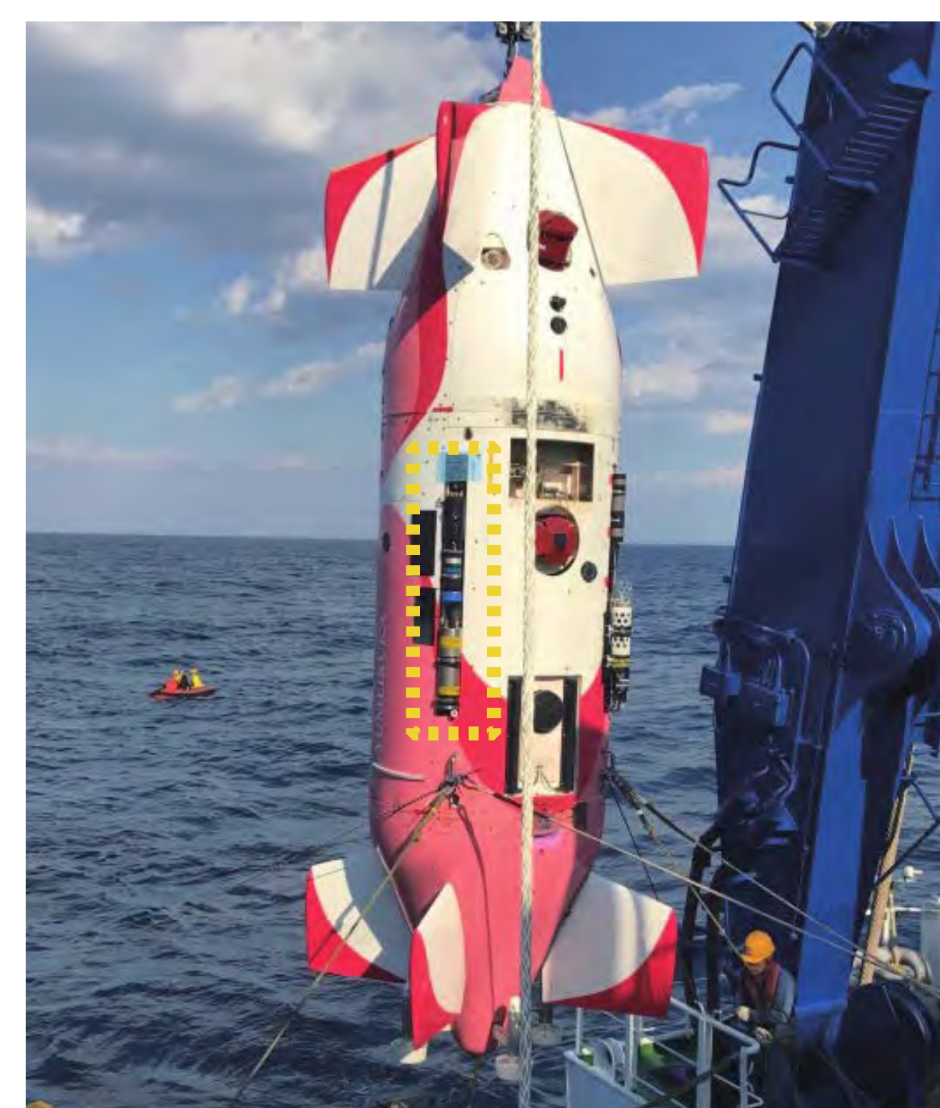
ATP analyzer mounted on Autonomous Underwater Vehicle
