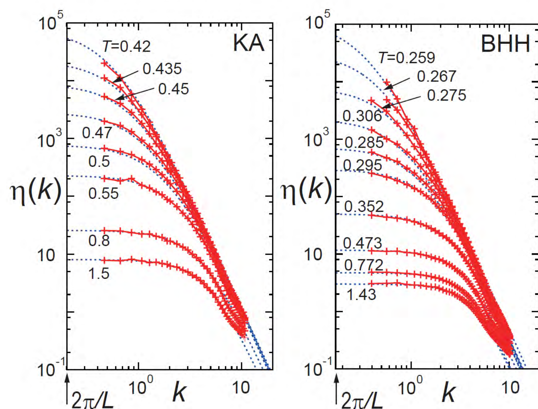
Wavenumber dependent shear viscosity
