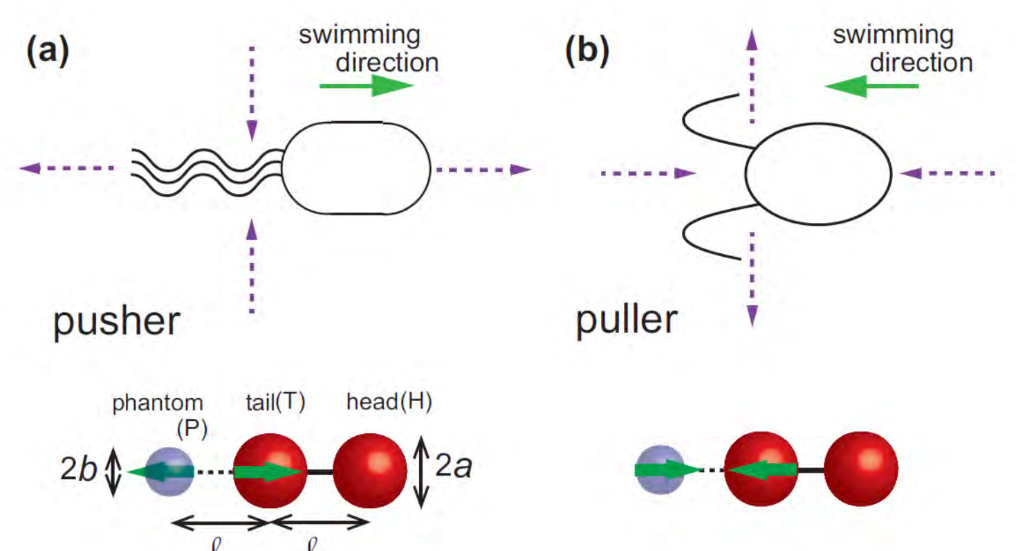
Minimal microorganism model
