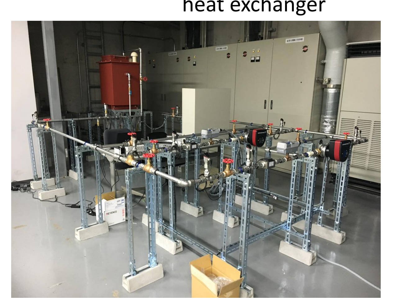
■ Experimental system of water transport system in HVAC
