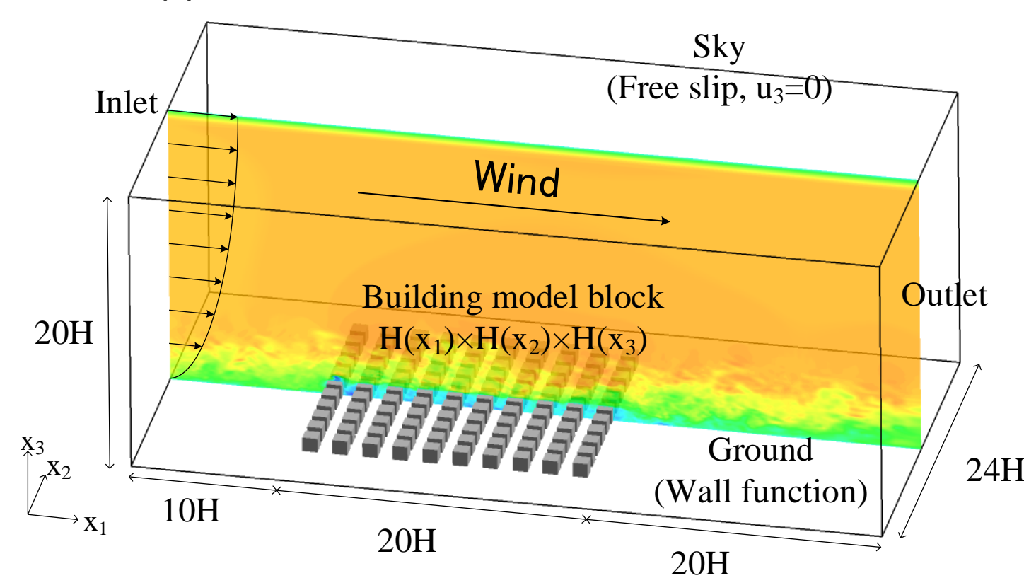
■ High-resolution analysis of urban air flow using LES
