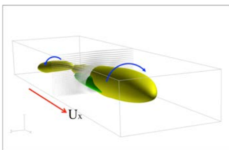
Fig.1 Vortex structure near the wall in turbulent channel flow
