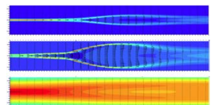
Fig.3 Current and jet of magnetic reconnection
