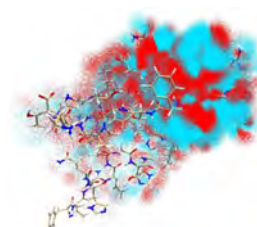
Highest occupied molecular orbital of insulin drawn by cloud-like model
