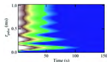
Rabi oscillation of quantum state
