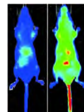
Fluorescent imaging of Vitamin C in a mouse
