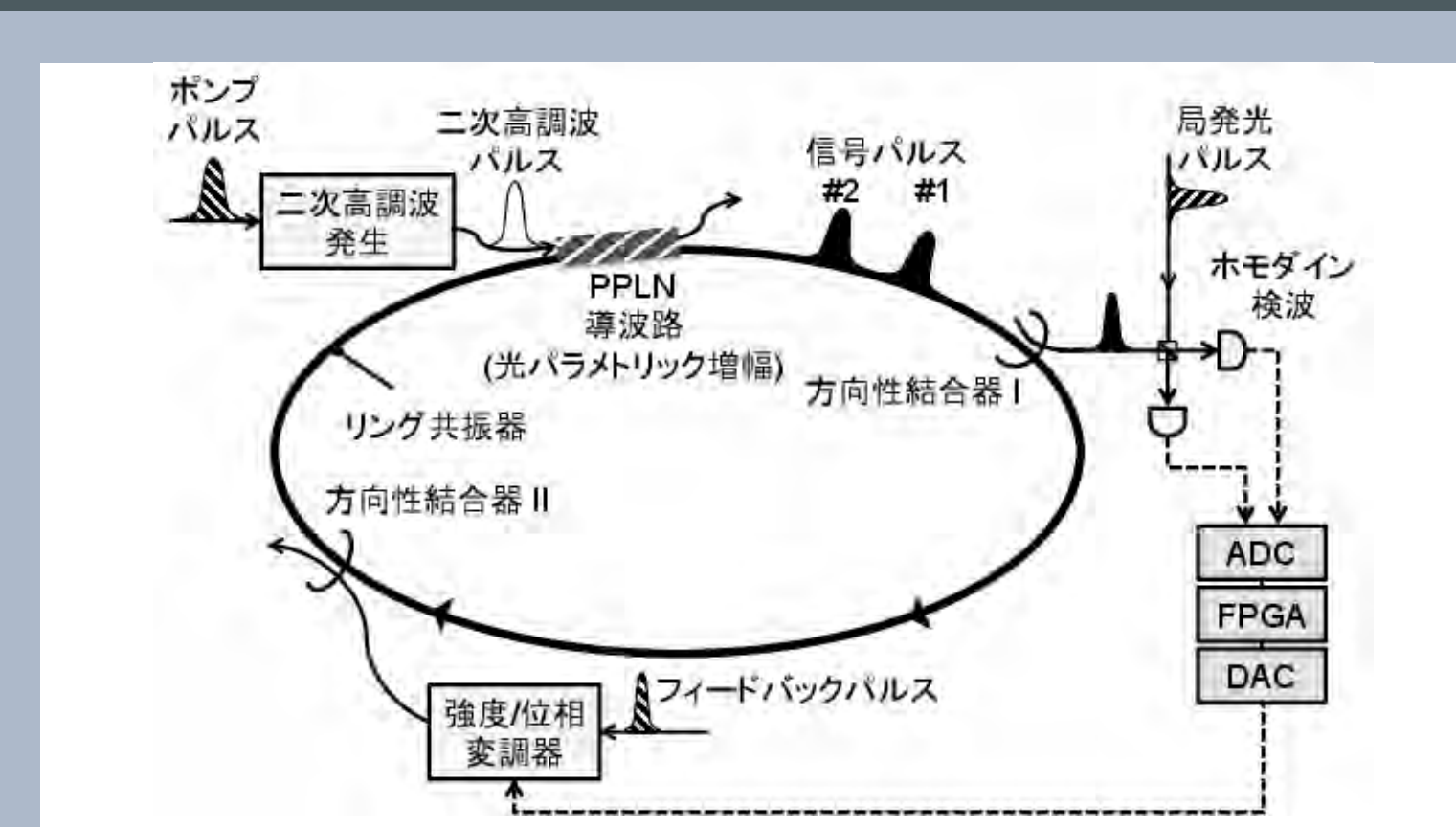
"Optoelectronic neural network" based on degenerate optical parametric oscillators
