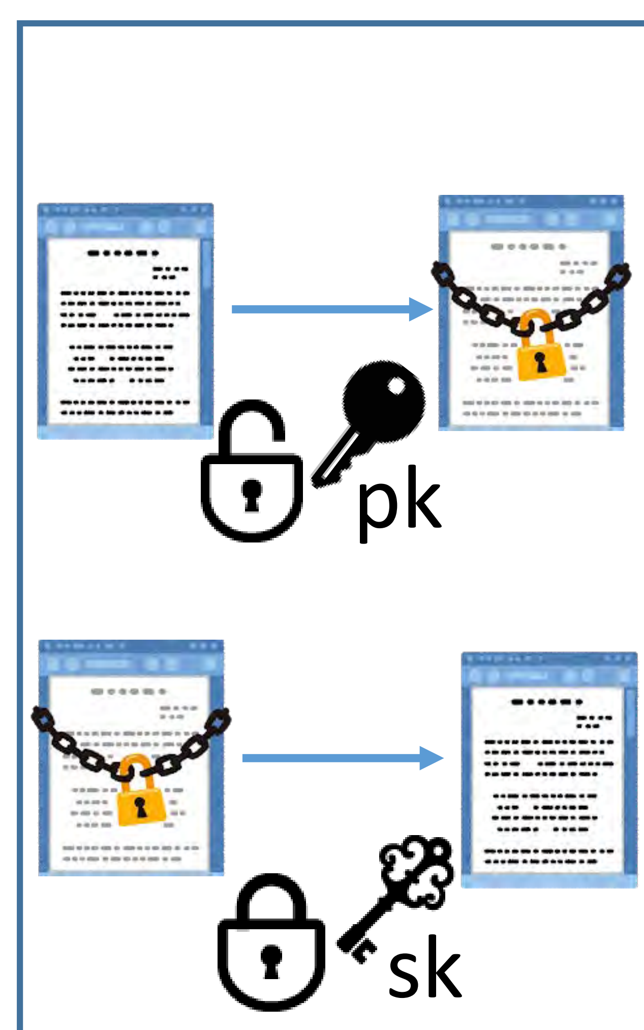
Public-Key Encryption
