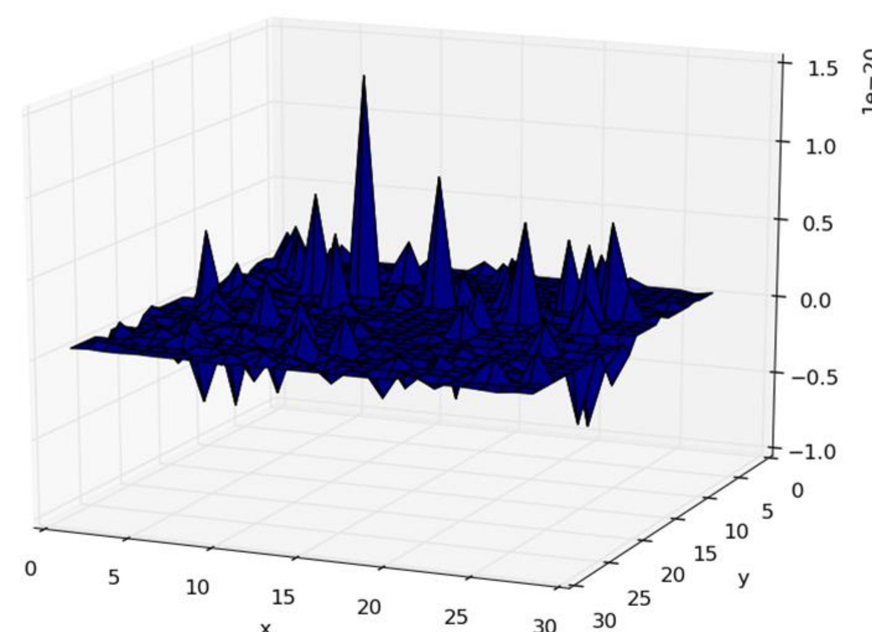
Saliency map
