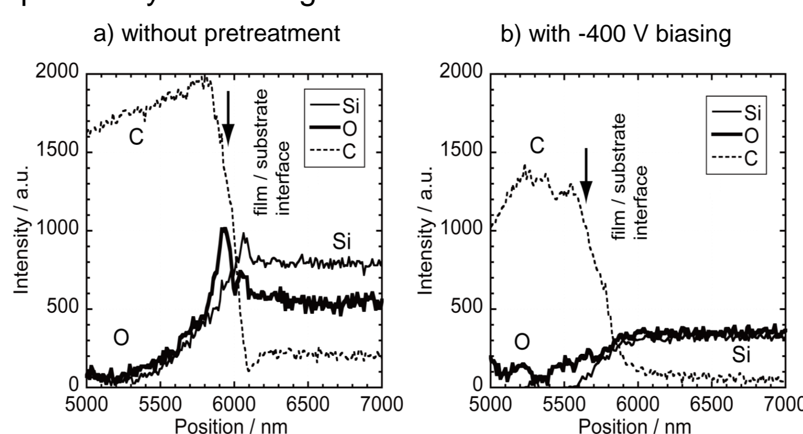
Depth profiles of the C, O, and Si measured by AES. Oxygen at the interface was removed by substrate sputtering before the deposition. The gradual change of the C concentration in the sputtered film (b) is indicative of the mixed layer of C and Si at the interface.
