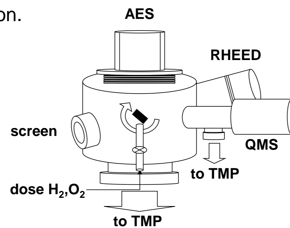
Schematic diagram of the surface analysis chamber. The base pressure <math>< 10^{-9}</math> Pa is achieved inside the chamber. AES, RHEED, QMS, and heated gas sources enable the surface modification and analyses of desorbed species
