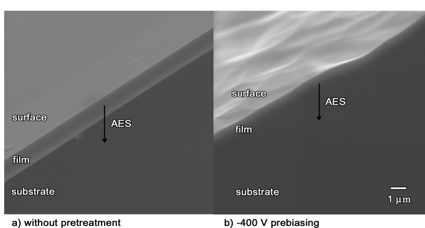
Cross sectional SEM images of DLC/Si interface. No clear interface between the substrate and the DLC film are identified in the film (b) deposited after a negative biasing to the substrate.
