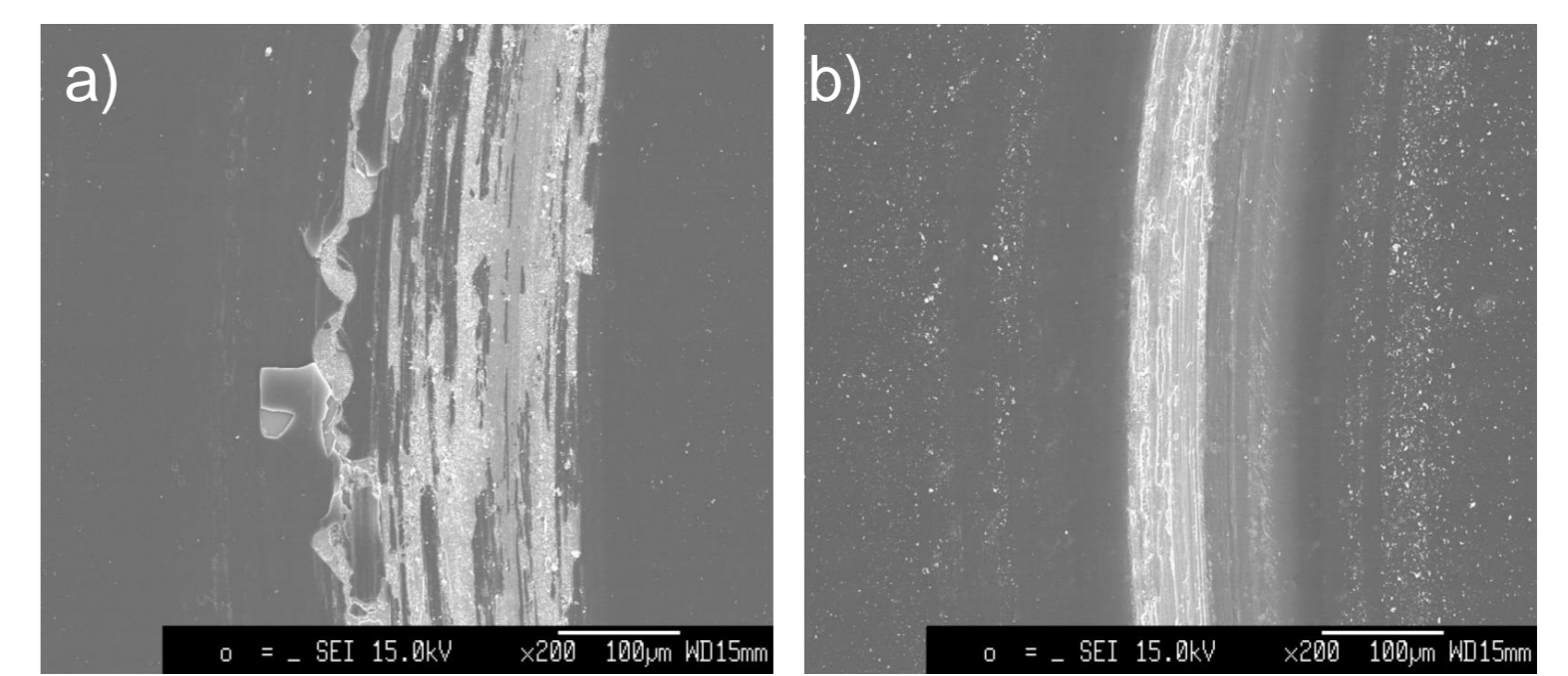
Traces of the ball on the DLC/AL components after ball-on-disk wear tests. The film delamination observed on the reference sample (a) was inhibited on the sample (b) deposited after pretreatment
