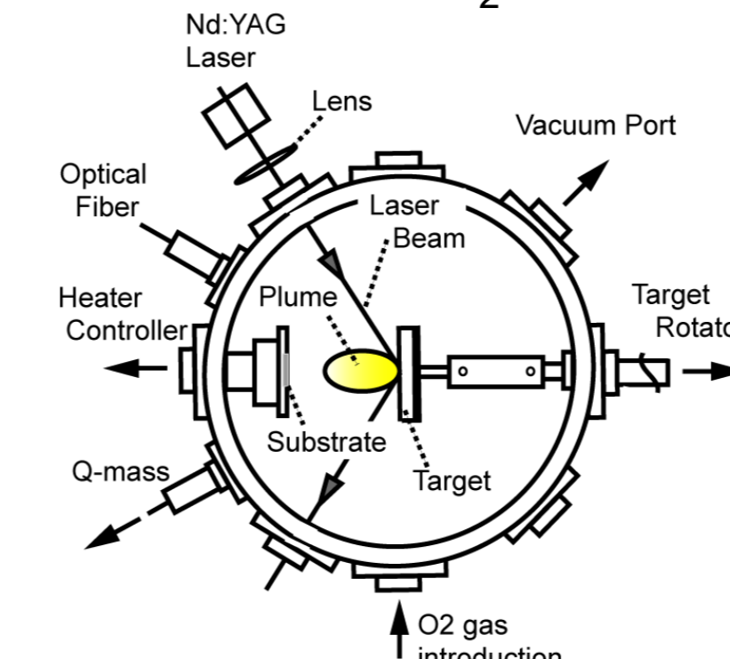
Pulsed-laser deposition chamber with a Nd-YAG laser. The base pressure reaches 10 -7 Pa.
