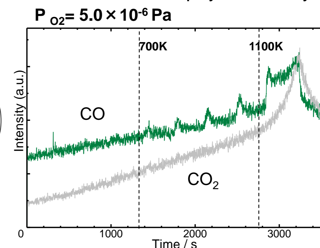
Desorption species from diamond during a thermal annealing in oxygen. Oxygen on the diamond surface is always detected as CO when it is removed from the surface.
