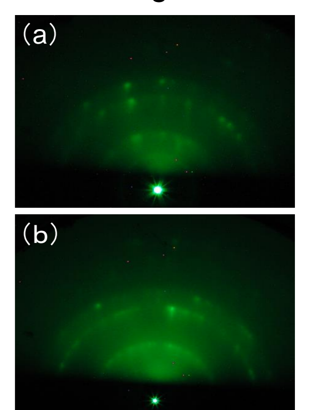
RHEED images of diamond surfaces (a) before and (b) after annealing in oxygen.
