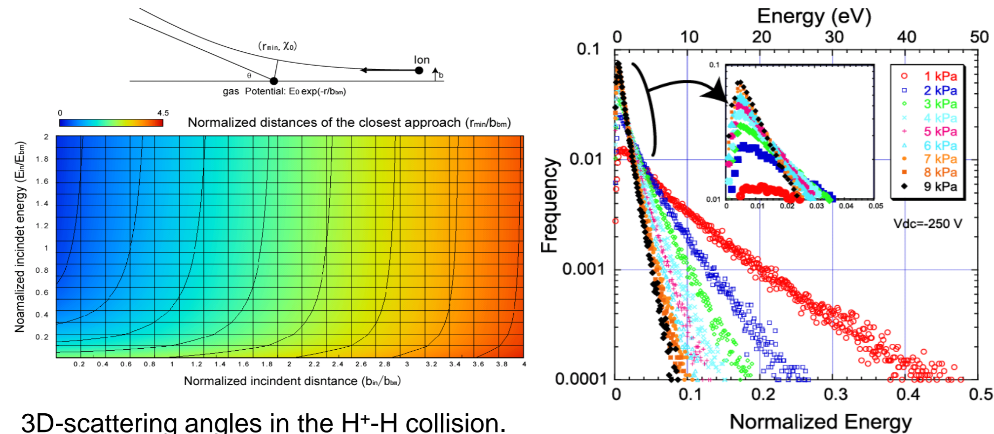
H + loses most energy in the sheath, i.e., plasma/substrate boundary.
