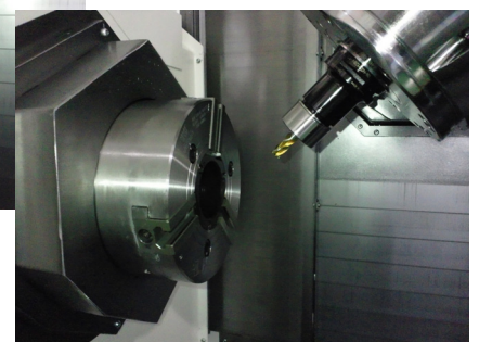
CNC TurningCenter
