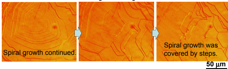
Growth interface during solution growth of SiC at 1400
