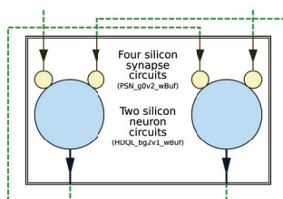
Fig.3 Silicon half-center oscillator chip
