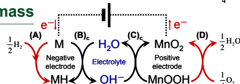
Schematic image of Fuel Cell/Battery System (upper) discharge (lower) charge
