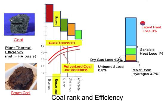
Coal rank and Efficiency
