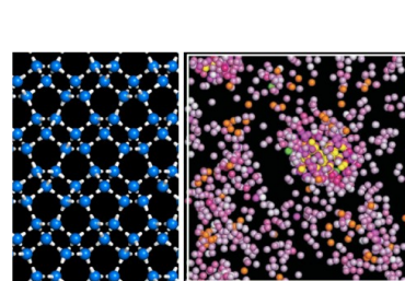
A newly discovered ice (left) and the birth of an ice crystal (light)
