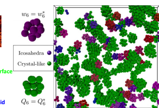
Locally ordered regions in a colloidal supercooled liquid near the glass transition (Reconstructed from experiments).
