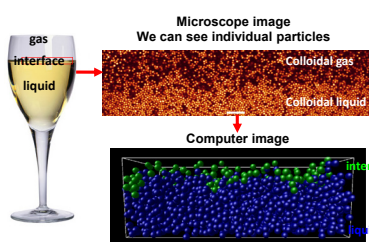
Single-particle-level observation of the gas-liquid interface of a colloidal fluid
